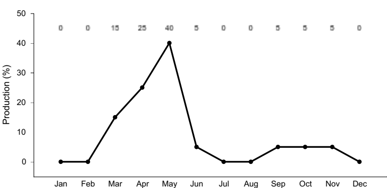
Figure 7. Plant community growth curve (percent production by month). ID0611, POSE/ BRTE/ ANNUALS . State 2.
