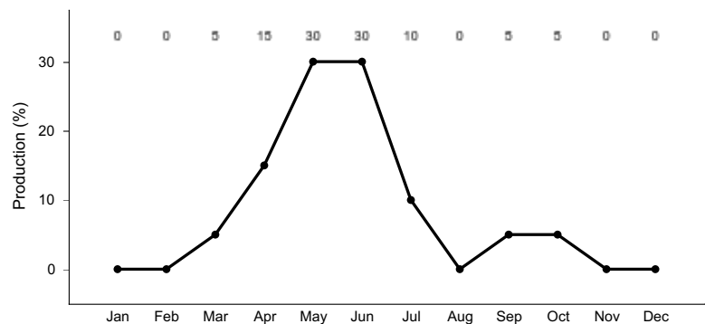
Figure 7. Plant community growth curve (percent production by month). ID0912, ARTRV-PSSP6 high elevation.
