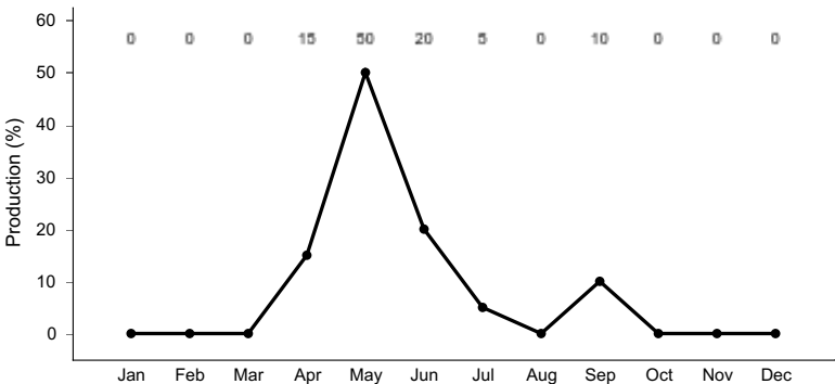
Figure 13. Plant community growth curve (percent production by month). WY0501, 5-9BH Upland sites. Monthly percentages of total annual growth for all upland sites with dominantly C3 Cool season plants..
