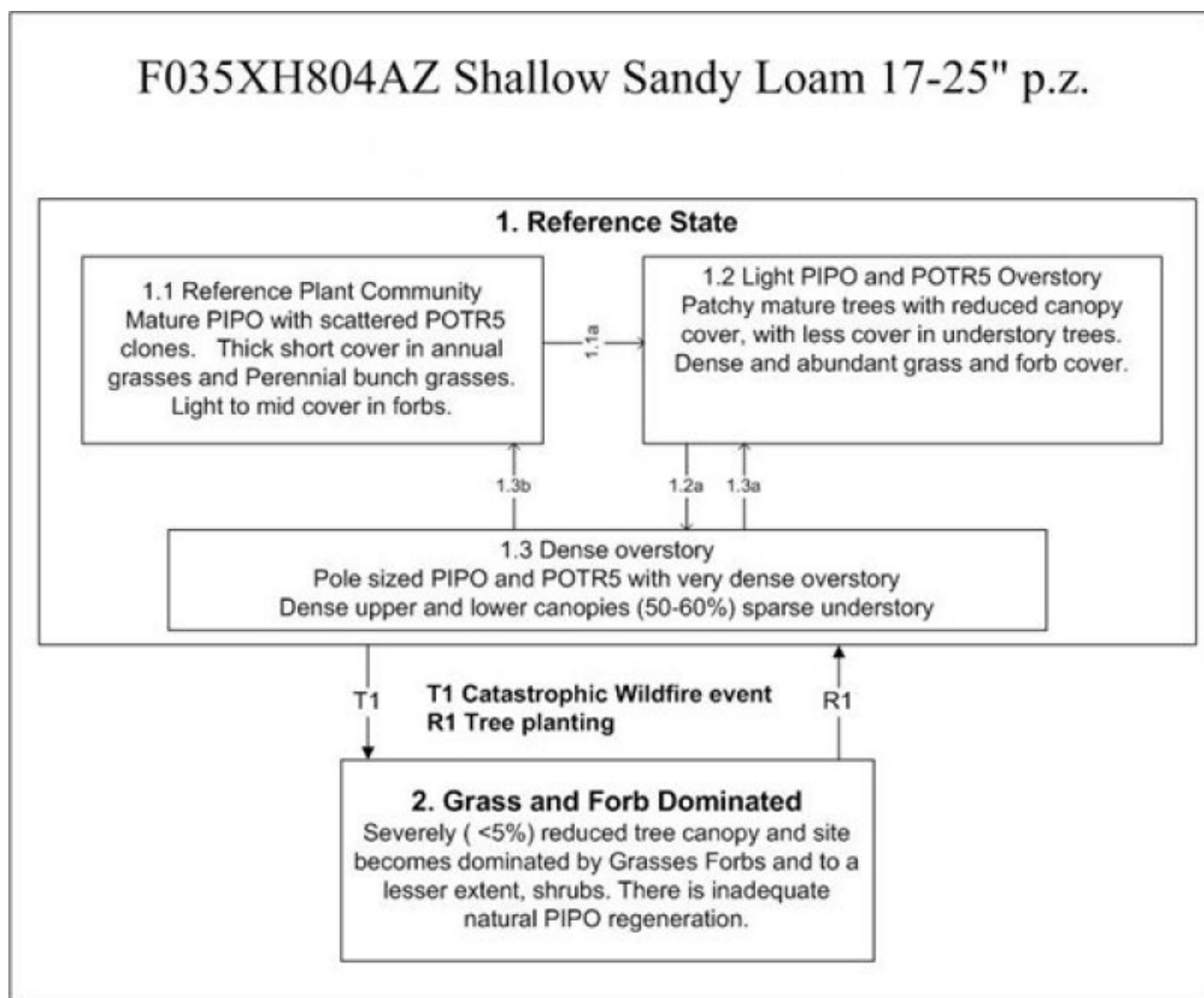
Figure 4. 358 ShallowSandyLoamS&T
