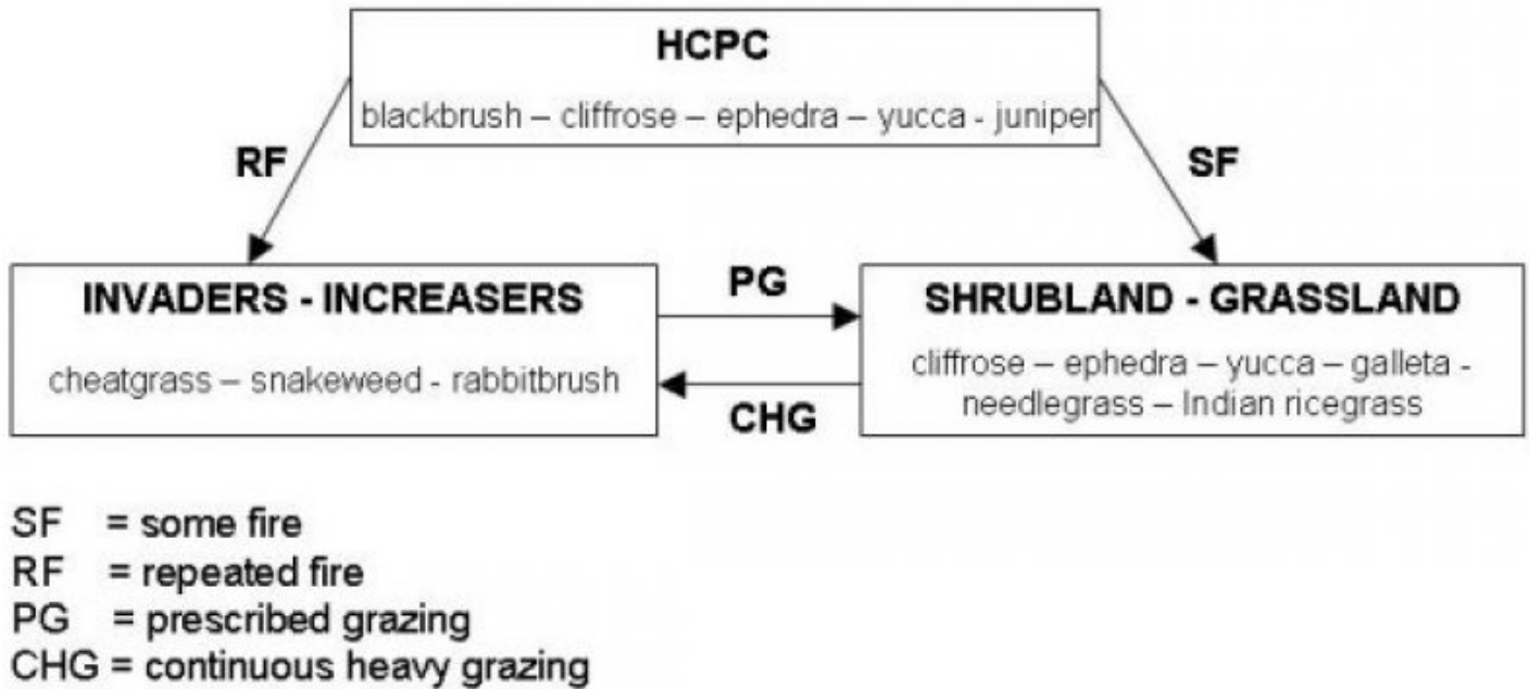
Figure 4. Basalt Slopes, calcareous 10-14" pz = 035XC340AZ
