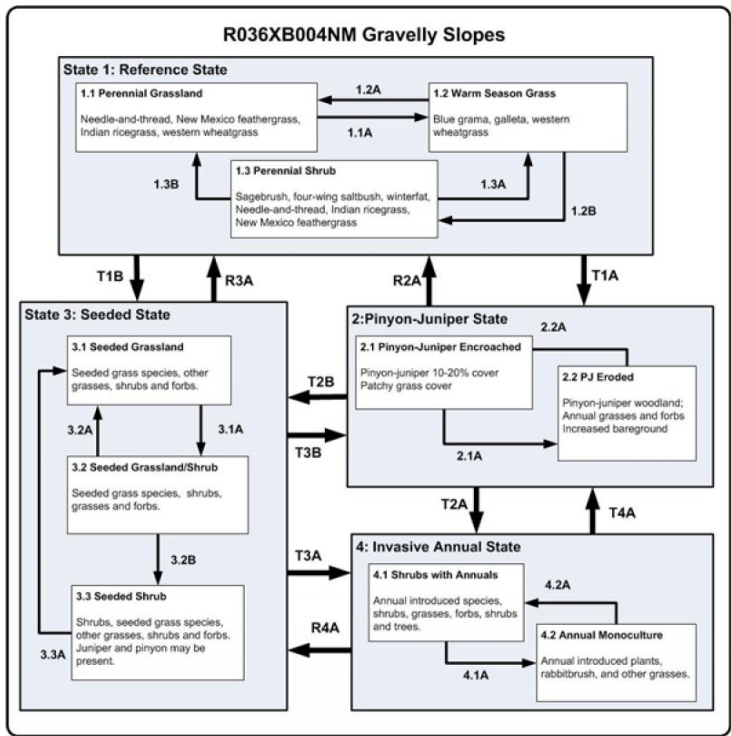
Figure 6. STM
