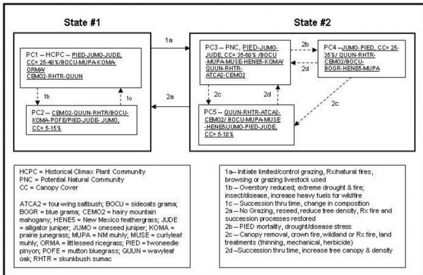
Figure 4. State-and-Transition Model
