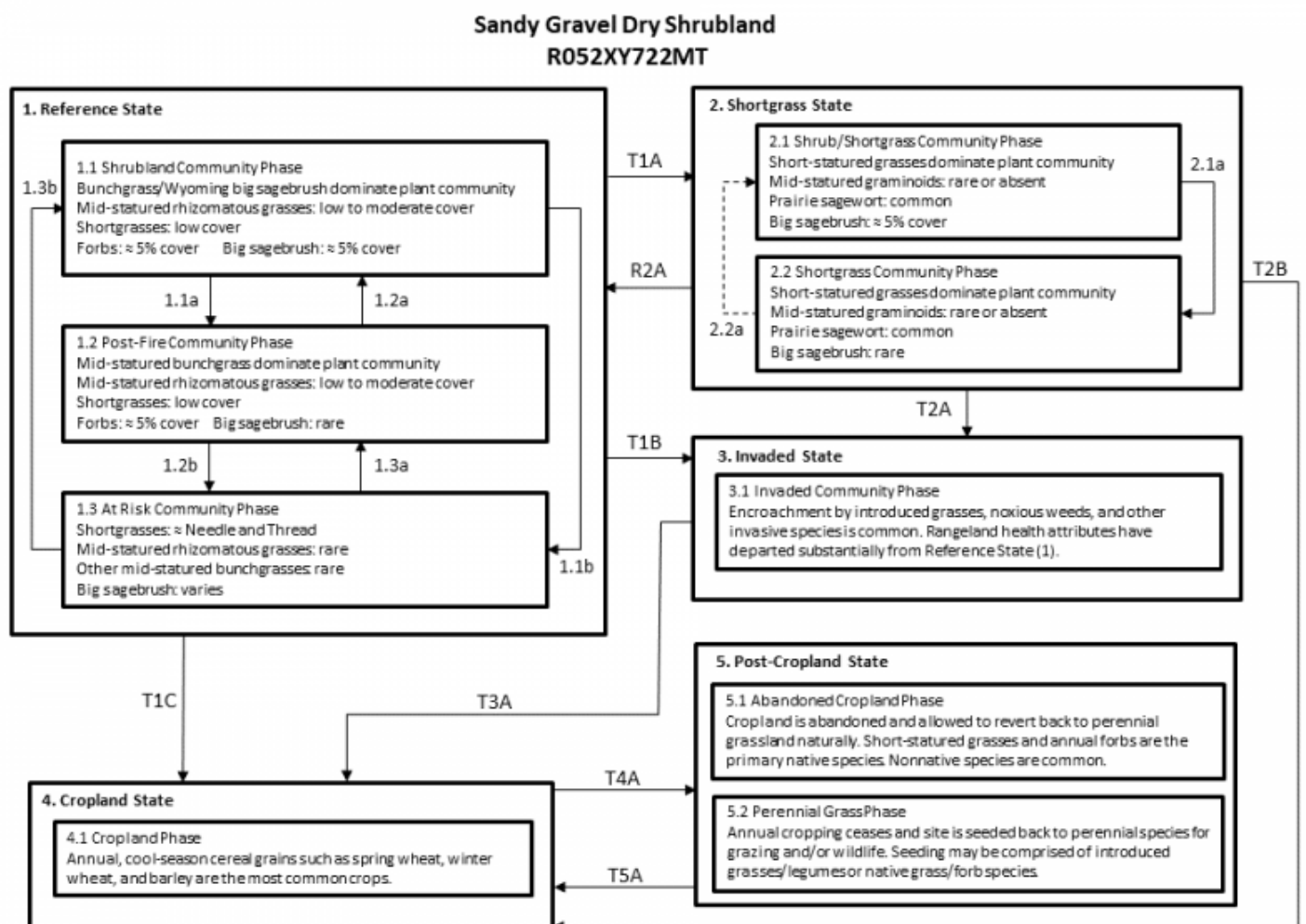
Figure 2. State-and-transition diagram.
