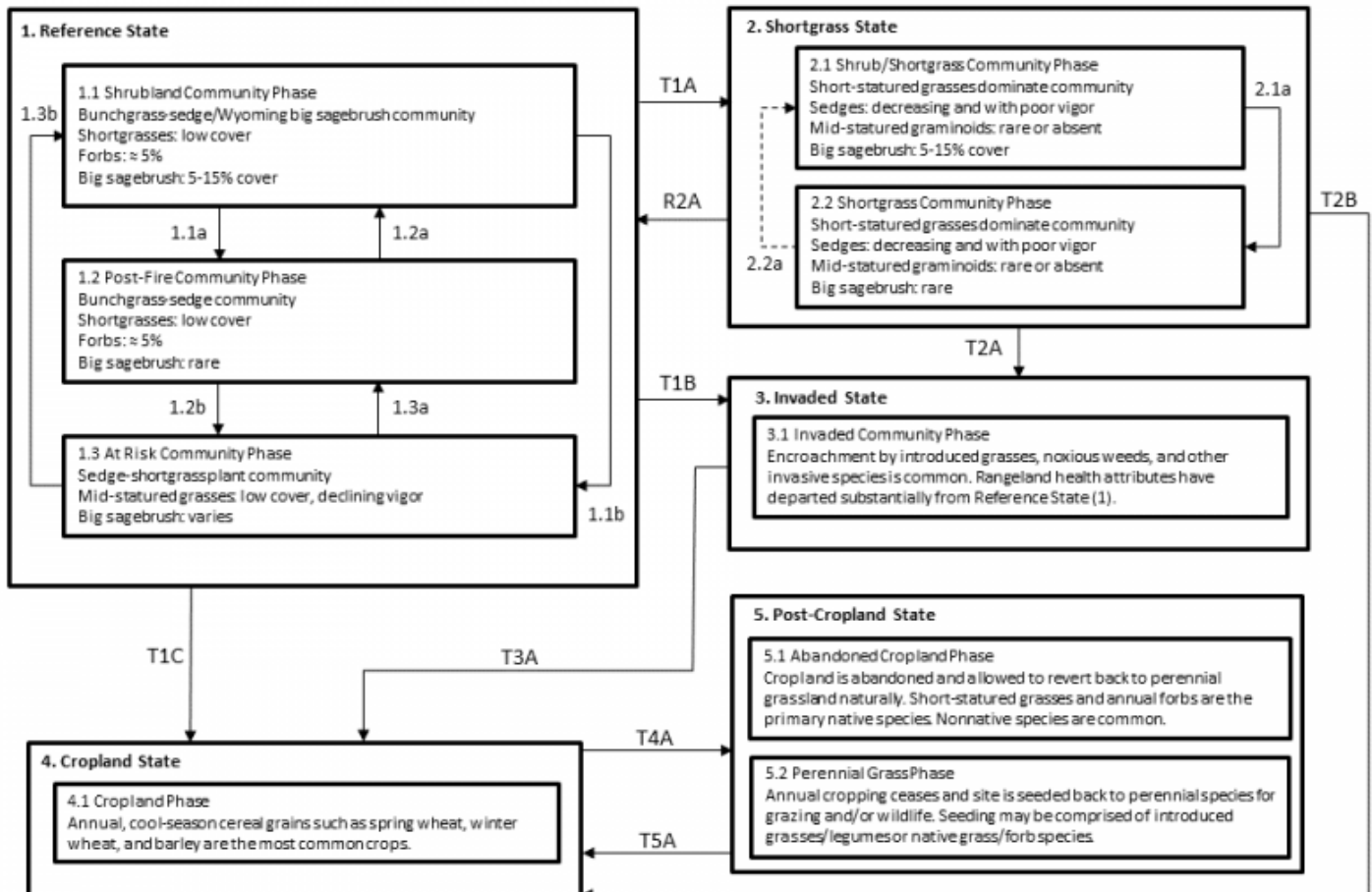
Figure 2. State-and-transition diagram.
