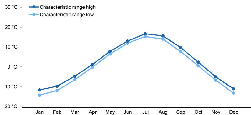
Figure 2. Monthly minimum temperature range
