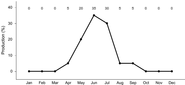
Figure 10. Plant community growth curve (percent production by month). WY1104, 12-14SP upland sites w/ warm. 12-14" Precipitation Zone, Southern Plains (SP) with warm-season (grass) species.
