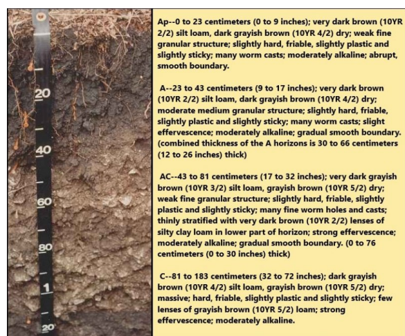
Figure 10. MLRA 76 Ivan soil series profile and description.
