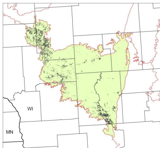
Figure 1. Distribution of Dry Sandy Bedrock Uplands in the Wisconsin Central Sands MLRA (89).
