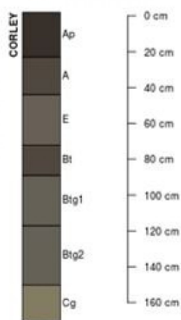
Figure 11. Figure 6. Profile sketch of soil series associated with Wet Upland Depression Prairie.
