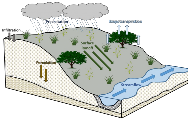
Figure 9. Figure 5. Hydrologic cycling in Till Upland Forest ecological site.
