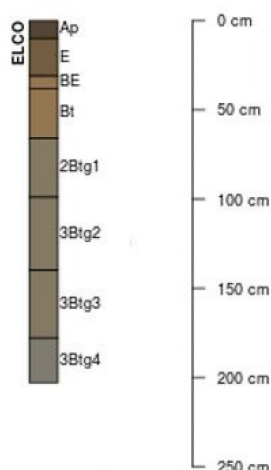
Figure 10. Figure 6. Profile sketches of soil series associated with Till Upland Forest.
