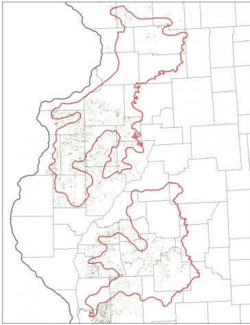
Figure 1. Figure 1. Location of Till Upland Forest ecological site within MLRA 108B.
