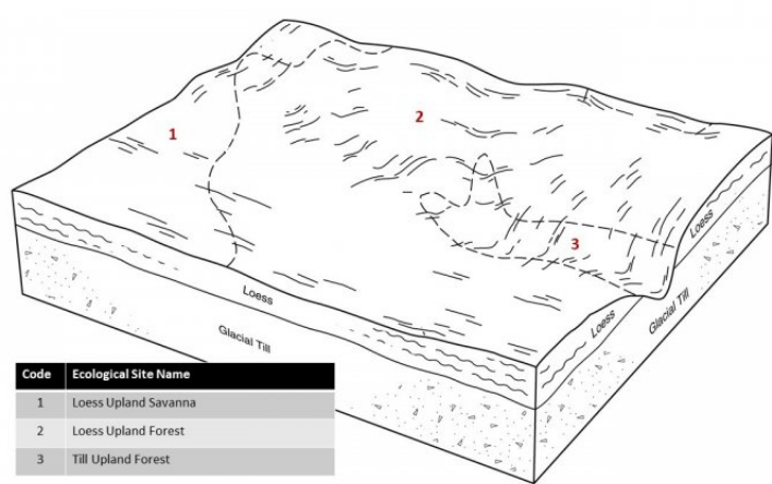
Figure 2. Figure 2. Representative block diagram of Till Upland Forest and associated ecological sites.
