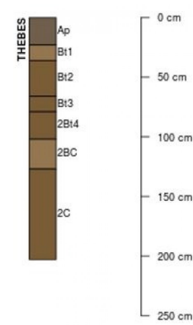
Figure 9. Figure 5. Profile sketch of soil series associated with Loamy Outwash Forest.
