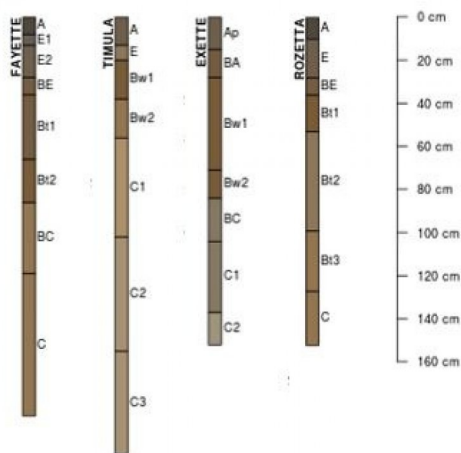
Figure 11. Figure 6. Profile sketches of soil series associated with Loess Upland Woodland.
