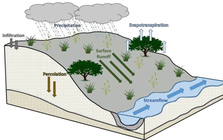
Figure 10. Figure 5. Hydrologic cycling in Loess Upland Woodland ecological site.
