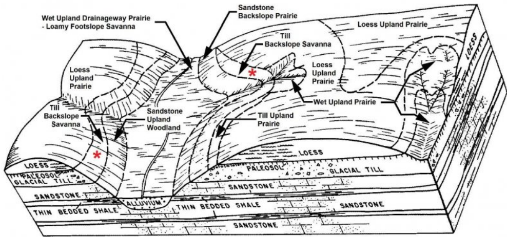
Figure 3. Block diagrams representing typical soil-landform sequences in Loess Ridges, Glacial Till Side/Footslopes. Red asterisks identify soil components correlated to Till Backslope Savanna.
