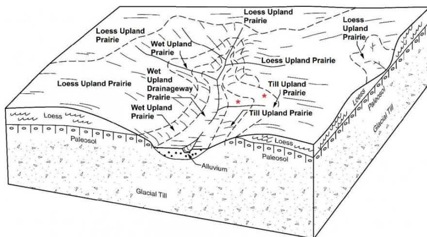
Figure 2. Block diagrams representing typical soil-landform sequences in A) loess ridges and B) loess ridges and glacial till side/footslopes. Red asterisks identify soil components correlated to Till Upland Prairies.
