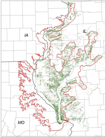
Figure 1. Location of Loess Protected Backslope Forest ecological site within LRU 115XC.
