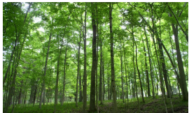
Moderately Deep Interbedded Limestone/Shale Maple Oak Forest
