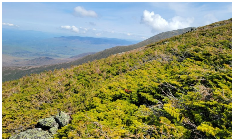
Figure 7. A high-elevation Black Spruce-Balsam Fir Krummholz on Mount Washington, New Hampshire. The stunted, wind pruned thickets are a result of the extreme climate, allowing for growth on the leeward side of prevailing winds. Photo taken May 17th, 2024.
