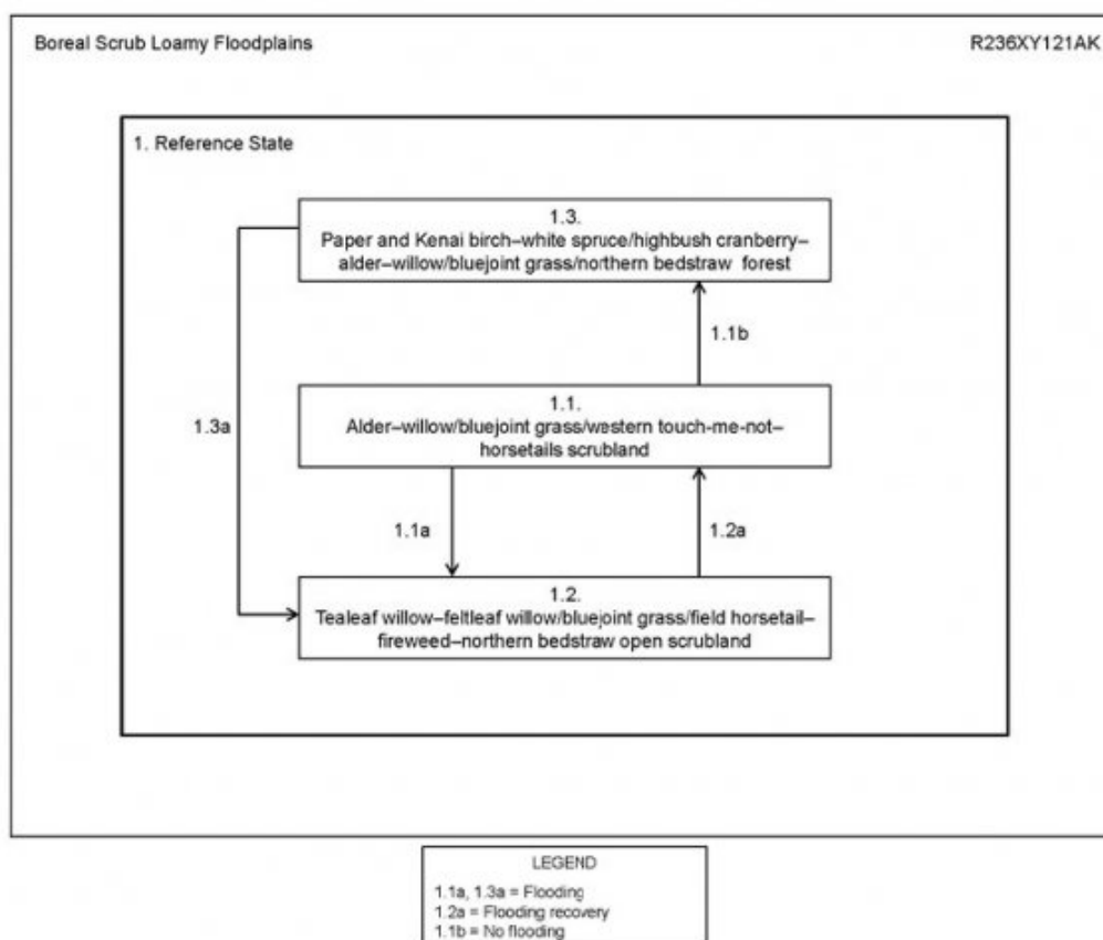
Figure 8. State-and-transition model.
