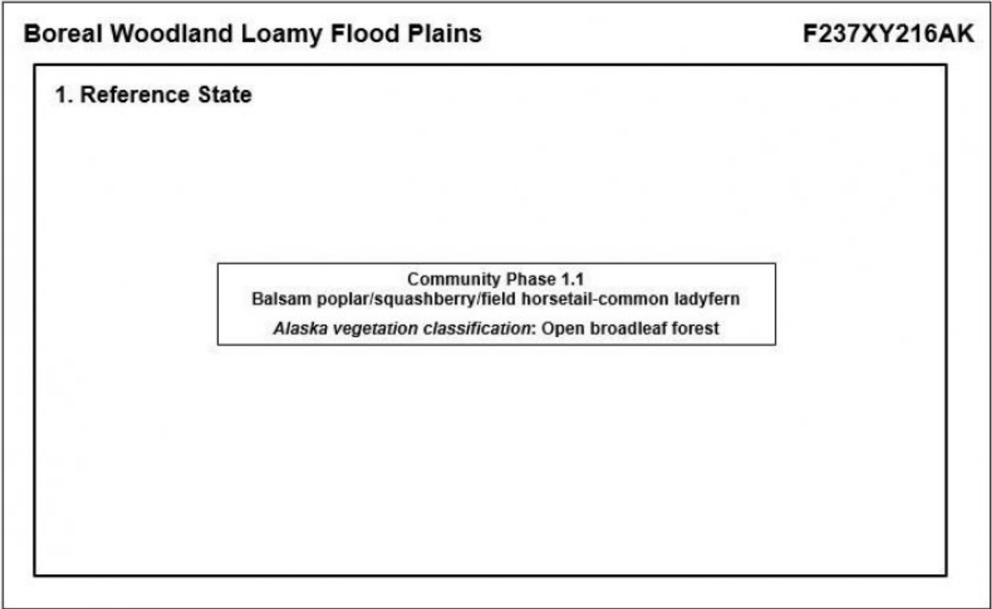
Figure 4. State-and-transition model.
