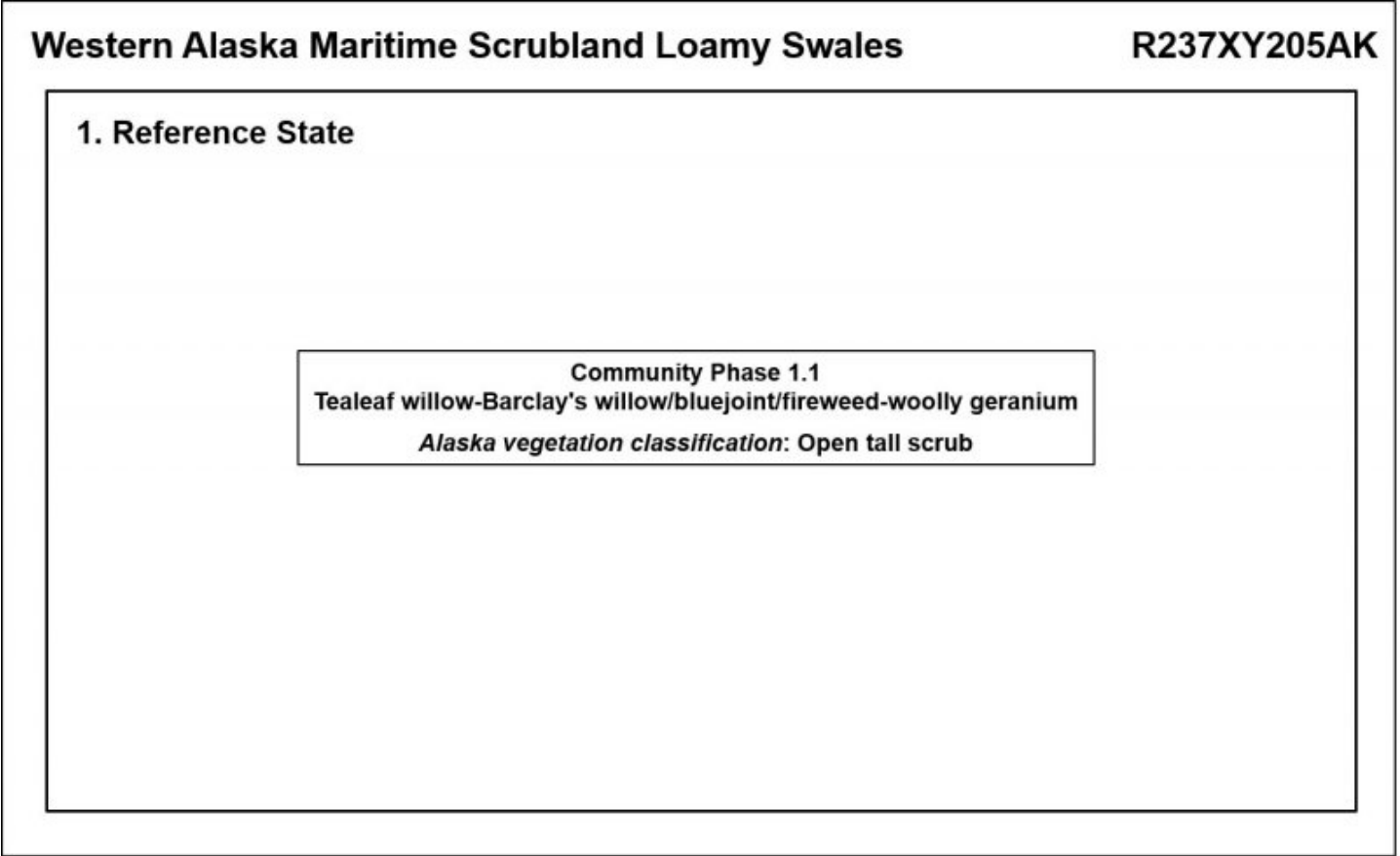
Figure 5. State-and-transition model.
